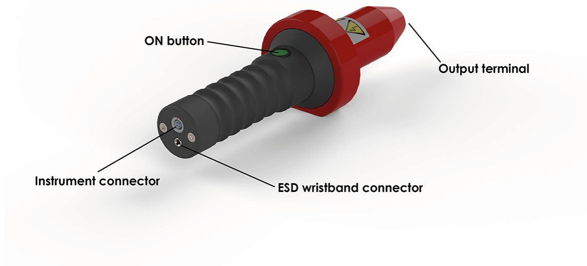
Fig 3 – Dry Roof Pro2 Handle
